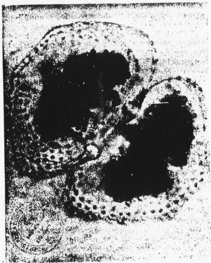
Chlorophyll Cell (algae) (The Universal Microscope). 17,000X on 35 mm. film.
